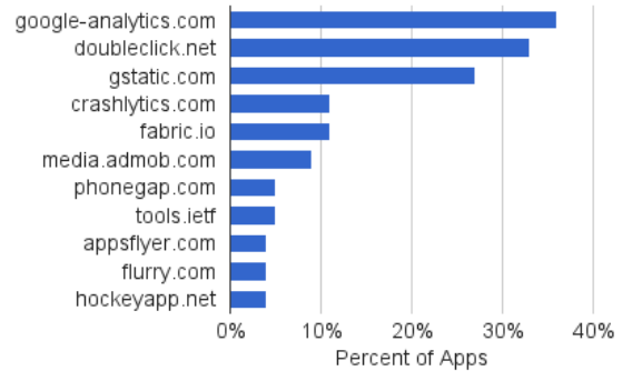
Figure 6: Most common ad libraries and 3rd-party libraries.
