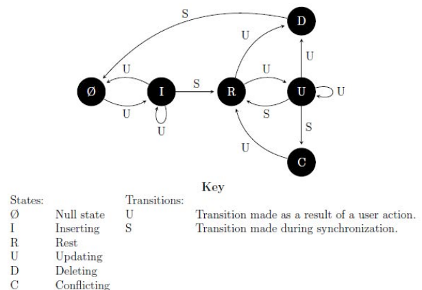
Figure 3: Synchronization state machine for a row in Tables.
