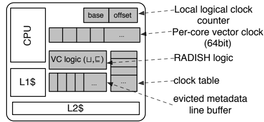
Figure 3.1: Overview of the RADISH processor core. State added by RADISH is shaded.
