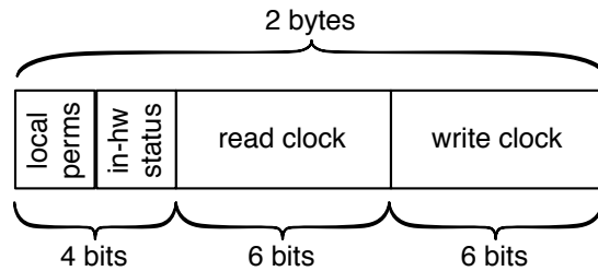
Figure 3.2: RADISH’s in-cache metadata format. Local permissions have 3 possible values, and in-hardware status 4 values, so we use 4 bits to represent the 12 combinations. 6 bits are left for each clock; we discuss rollover issues in [38].
