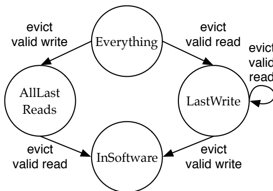
Figure 3.4: In-hardware status is downgraded when metadata is evicted from the last-level cache.
