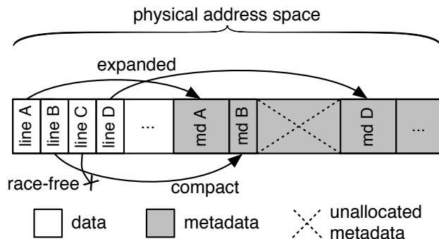
Figure 3.3: Mapping from data to metadata addresses for a single processor. Each processor uses a distinct portion of the physical address space.
