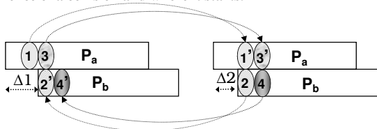
Figure 6: ZigZag decodes then re-encodes a chunk. Before subtracting a decoded chunk, like chunk 1, ZigZag needs to re-encode the bits to create an image of chunk 1’, as received in the second collision.
