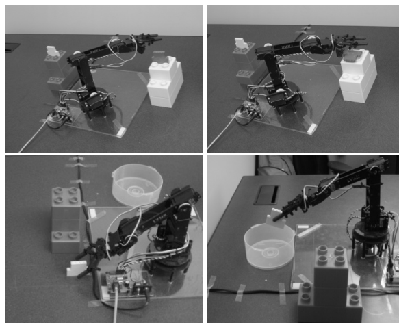
Figure 5: The simple and intermediate online tasks. The first row shows the simple task, where the robot arm starts in the middle, and the goal is to topple the two objects placed on either side. The second row shows the intermediate task, where the goal is to pick up a designated object, carry it over an obstacle, and drop it in the bin.
