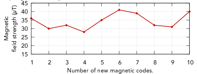
Figure 12: Reprogrammability of magnetized fabric. Adding new data to the same fabric strip has no substantial effect on its ability to store data.
