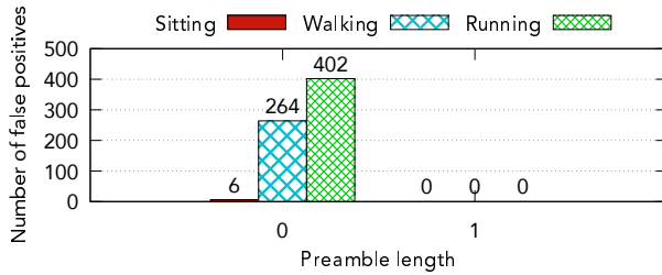
Figure 18: False positives in different settings. A preamble length with just one gesture reduces false positives to zero in all three conditions.
