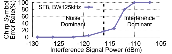
(b) Orthogonal Transmissions with Different Received Signal Power. We set the power of LoRa transmission with BW_1 = 125kHz to -123 dBm and increase the power of the other one.
