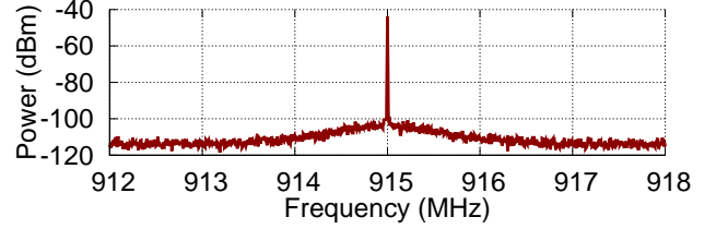
Figure 8: TinySDR Single-Tone Frequency Spectrum.
