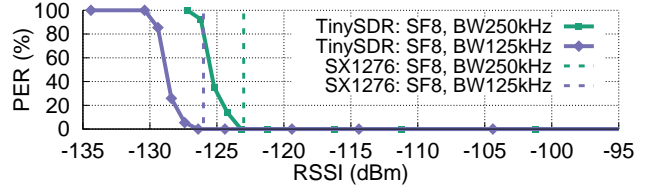
Figure 10: LoRa Modulator Evaluation. We evaluate our LoRa modulator in comparison with Semtech LoRa chip.
