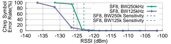
Figure 11: LoRa Demodulator Evaluation. We evaluate our LoRa demodulator by demodulating chirp symbols at different RSSI.
