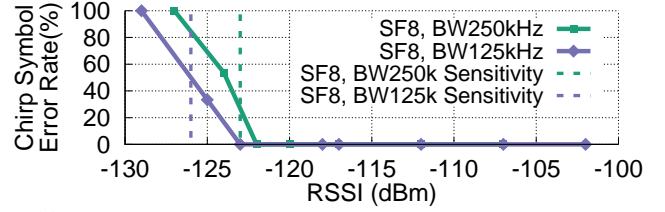
(a) Orthogonal Transmissions with Same Received Signal Power.
