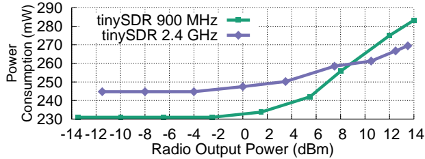
Figure 9: Single-Tone Transmitter Power Consumption. We show the total power consumption of tinySDR including I/Q radio, FPGA, MCU and regulators at different transmitter output power. This is 15-16 times lower power consumption than the USRP E310 embedded SDR.
