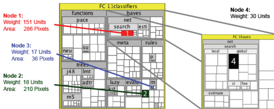
Figure 11. Existing treemap layout algorithms ignore the space dedicated to presenting structure. This leads to a distortion of node sizes and the notable complete absence of nodes. In this example, generated by the University of Maryland’s reference Treemap implementation [31], there are gross disparities between the weights and the space allocated to Node 1, Node 2, and Node 3. Even worse, Node 4 has almost twice the weight of Node 2 or Node 3, but is not visible in the treemap with first zooming into Node 1.
