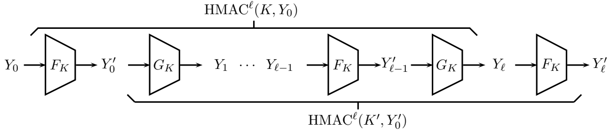
Figure 8: Diagram of two hash chains (K, Y) = (Y_0, \dots, Y_\ell) and (K', Y') = (Y'_0, \dots, Y'_\ell) for HMAC where \rho(K') = \rho(K) \oplus \text{xpad} .
