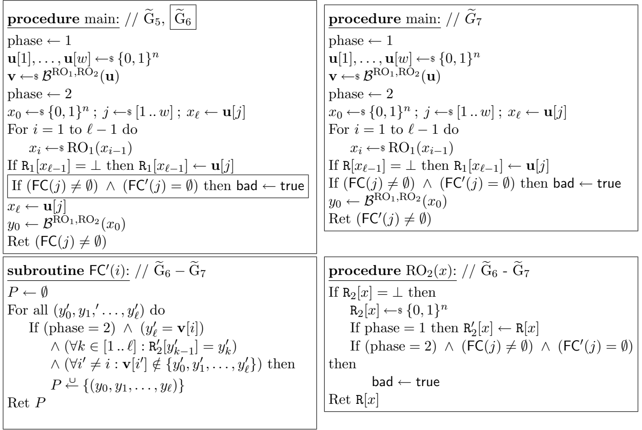
Figure 18: Descriptions of Games \tilde{G}_5 - \tilde{G}_7 .
