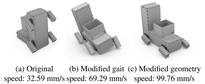
Figure 1. A robot design that topples while walking (a) can be modified to follow a gait that only wobbles slightly (b), but changing the geometry (c) allows the robot to move much faster and more steadily.
