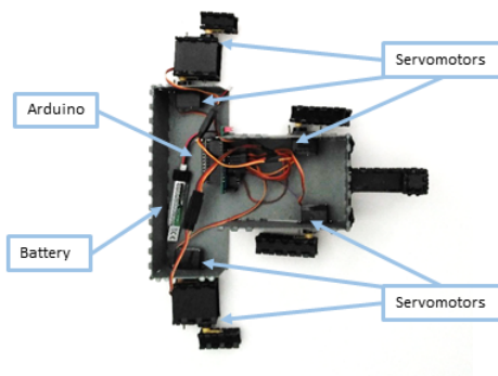
Figure 17. The electronics (servomotors, microcontroller, and battery) inside the Monkey example (Figure 16(d)).
