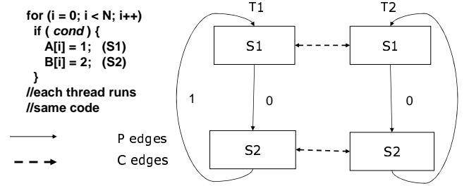
Fig. 5. SPMD Code for which Algorithm 3 Is More Accurate Than Algorithm 1
