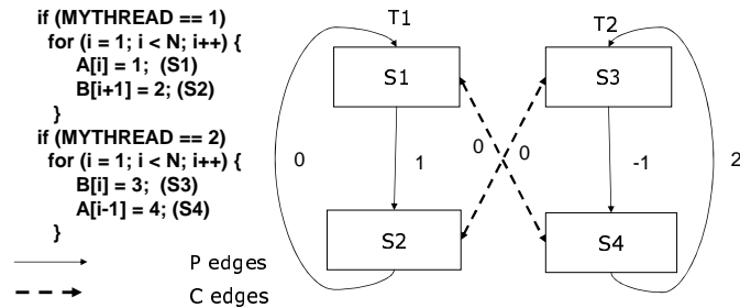
Fig. 4. Adding Edge Weights for Cycle Detection
