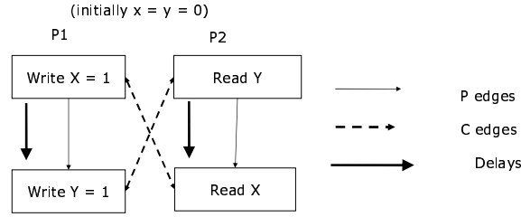
Fig. 2. Computing the Delay Set
