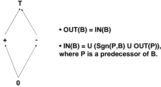
Fig. 6. Lattice and Flow Equations for Algorithm 4
