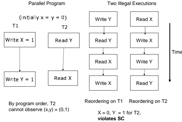
Fig. 1. Violation of Sequential Consistency: The actual execution may produce results that would not happen if execution follows program order.
