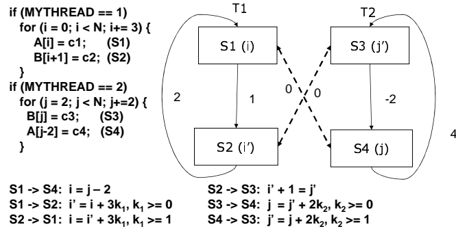
Fig. 3. Conflict Graph with Corresponding Constraints
