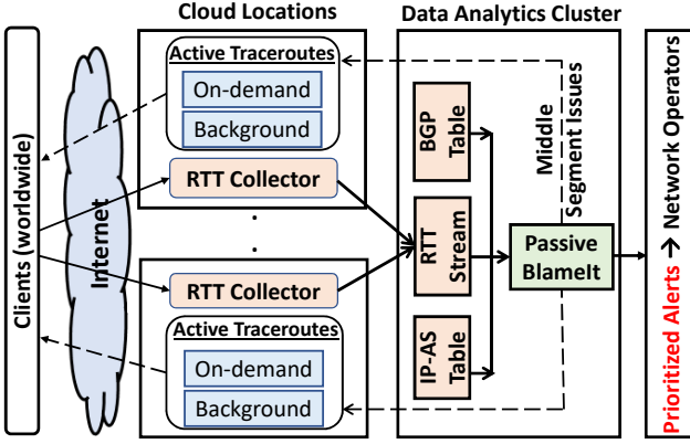
Figure 7: BlameIt’s key components in production.
