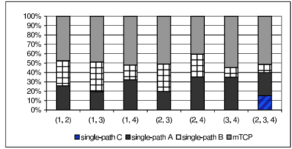
Figure 4: Throughput percentage of individual flows
