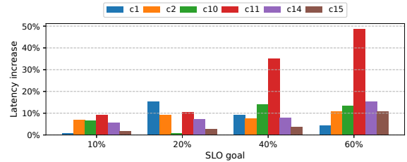
Figure 12. SLO maintenance under different thresholds.
