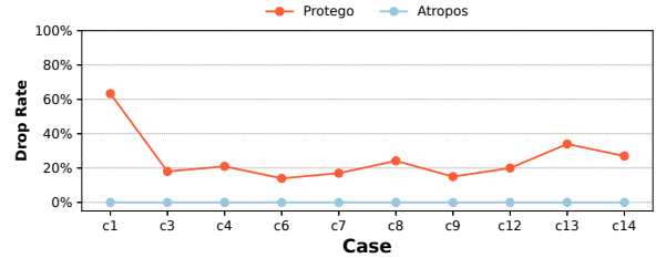
Figure 11. Drop rate of ATROPOS and Protego.
