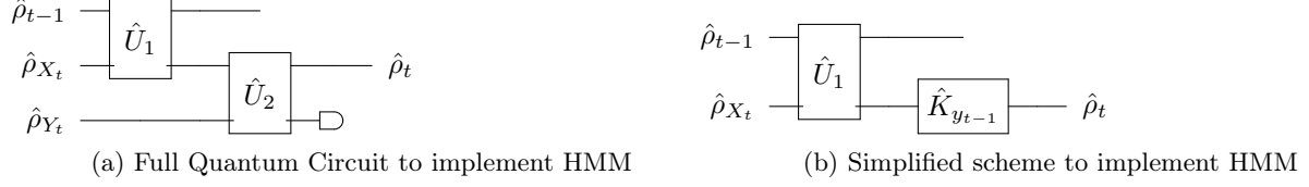
Figure 2: HMM implementation on quantum circuits
