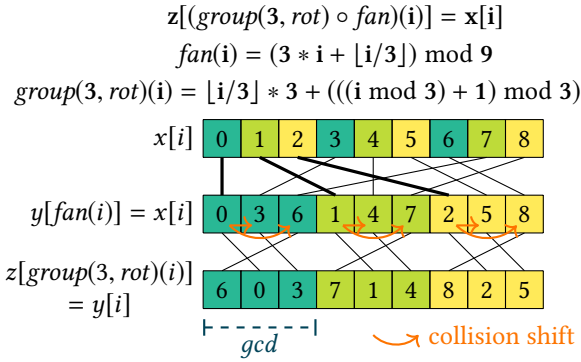
Figure 7. When swizzle expression is fanning followed by grouped rotation. n = \tilde{g}s = 9 , \tilde{c}_f = 3 , \tilde{d}_f = n/\text{gcd} = 3 , R = 1 , \overline{wrap} = \text{true}
