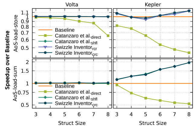
Figure 13. AoS-load-store and AoS-load-sum speedup when varying struct sizes. 2 Note that Swizzle Inventor cre is on top of Swizzle Inventor rer and Catanzaro et al. shfl .
