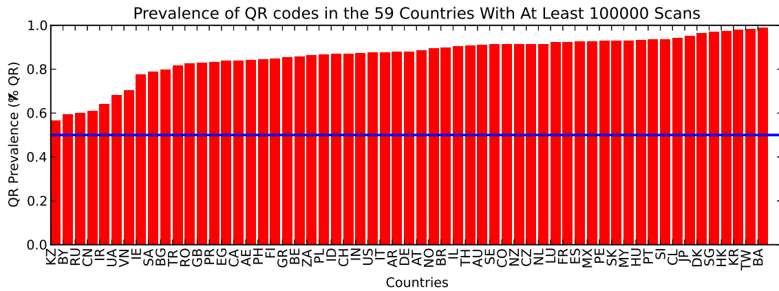
Figure 11: Percentage of scans which were of QR codes (as opposed to 1D barcodes) per country for the most scanning countries. The blue line indicates the y-coordinate for 50% QR codes—all countries with at least 100,000 scans are above the line and performed predominantly QR code scans.
