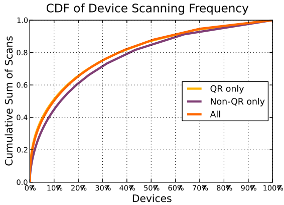
Figure 4: The distribution of scans across devices. Devices had nearly identical distributions of scanning for QR codes and all codes combined — the yellow (QR only) and orange (All) lines overlap almost entirely. The right hand side of the figure shows 30% of devices which contributed only one scan each. Heavy hitters on the left: 10% of devices performed half the total scans in the dataset.
