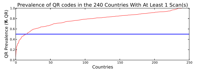
Figure 10: Percentage of scans which were of QR codes (as opposed to 1D barcodes) per country for all countries. The blue line indicates the 50% QR mark — countries below the line performed more 1D barcode scans than QR code scans, whereas countries above the line performed predominantly QR code scans. 6 out of 15 of these 1D dominated countries had fewer than 1000 total scans in the database, and none of the 15 had more than 51,000 scans.
