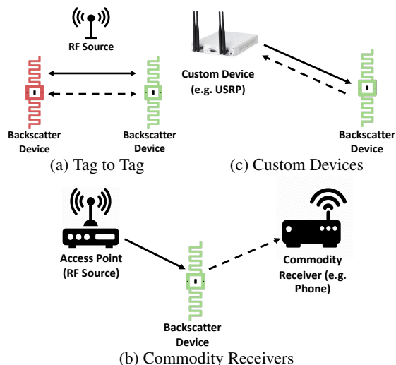
Figure 4: Prominent backscatter architectures.
