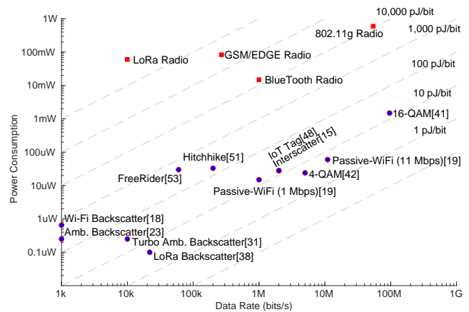
Figure 1: Energy efficiency. We plot power consumption of various radio and backscatter communication technologies as a function of data rates. The dotted lines represent constant energy efficiency.
