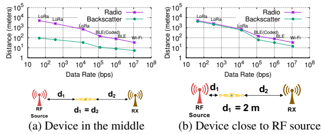
Figure 3: Operating distances. We compare radios with two backscatter deployments.
