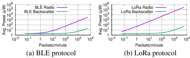
Figure 2: Power consumption versus duty cycling. We compare BLE and LoRa radios and their backscatter counterparts.
