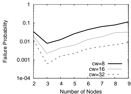
(a) With every node picking from a constant Congestion Window ( cw )
