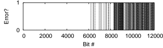
(a) Error Distribution due to Residual \delta f .
