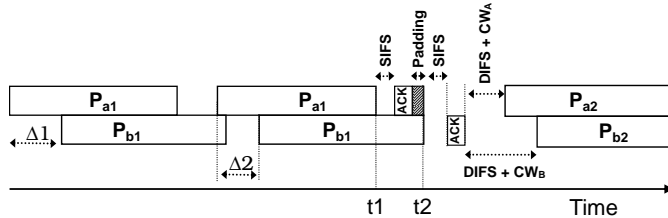
Figure 4-5 – ACKing. The figure shows how ZigZag can send 802.11 synchronous acks.
