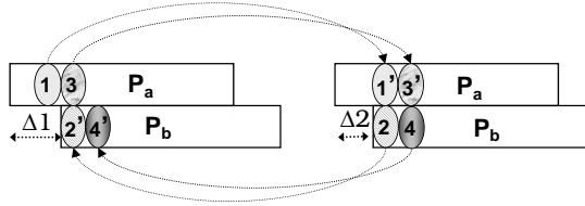
Figure 4-3 – ZigZag decodes then re-encodes a chunk. Before subtracting a decoded chunk, like chunk 1, ZigZag needs to re-encode the bits to create an image of chunk 1', as received in the second collision.
