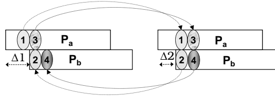
Figure 1-2 – ZigZag Decoding. ZigZag decodes first chunk 1 in the first collision, which is interference free. It then subtracts chunk 1 from the second collision and decodes chunk 2, which it can then subtracts from the first collision and decodes chunk 3, etc.
