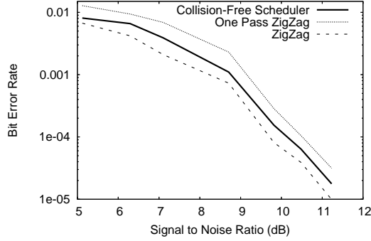
Figure 5-3 – Comparison of Bit Error Rate (BER). ZigZag delivers packets that are as correct as if they were sent in separate time slots. Further, if both backward and forward decoding are used, the BER is lower than if collisions did not occur.
