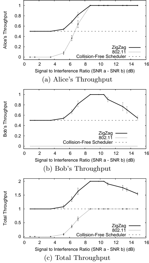
Figure 5-4 – Normalized Throughput in Scenarios with Capture Effects. The figure plots the throughput of the hidden terminals Alice and Bob, as Alice moves closer to the AP, i.e., as SINR \approx SNR_A - SNR_B increases. It shows that ZigZag achieves higher throughput than both 802.11 and the Collision-Free Scheduler. ZigZag is also fairer than current 802.11 where Bob cannot get any packets through.
