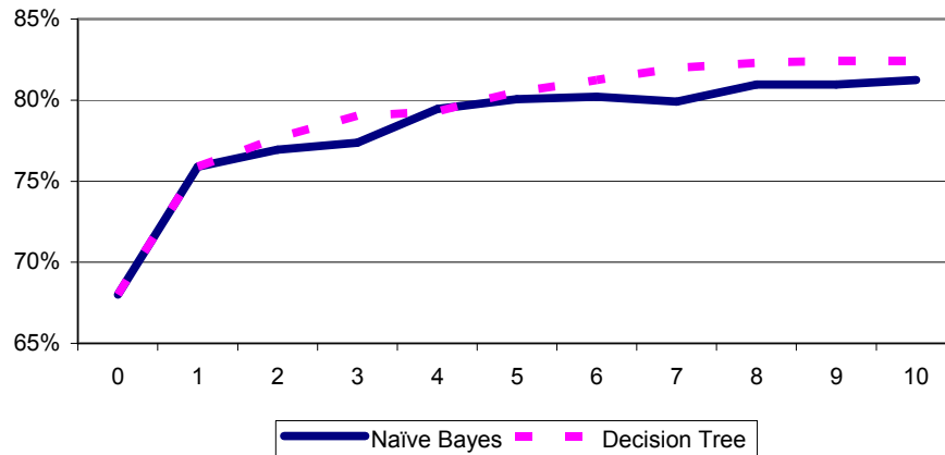
Figure 8 – Classifier accuracy versus number of features.
