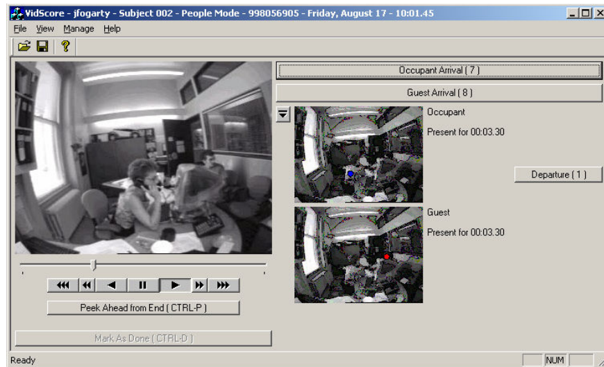
Figure 7 – Custom interface used for Wizard of Oz sensor simulation.
