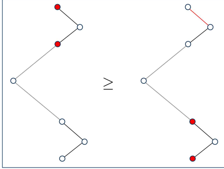
Figure 5: The main inequality on LRTs.
