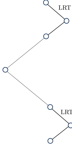
Figure 4: Two LRTs marked in a segment of a root-leaf path.
