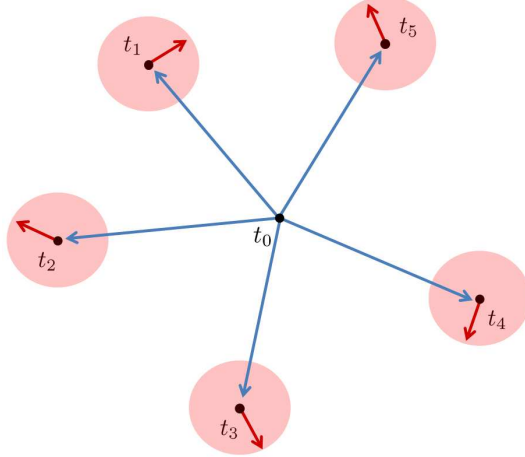
Figure 3: A “chaining” lower bound.
