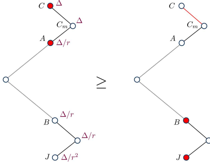
Figure 7: Proving the LRT inequality.
