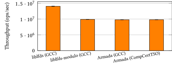
Figure 12. These are performance results for liblfdts’s lock-free queue vs. the corresponding code written in Armada. The Armada version, and our variant liblfdts-modulo, use modulo rather than bitmask operations. Each data point is the mean of 1,000 trials; error bars indicate 95% confidence intervals.
