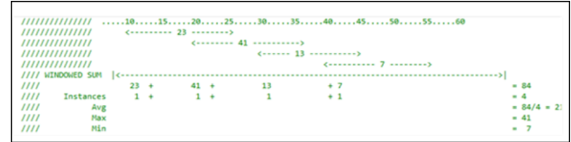
Figure 6. This comment, embedded in a sample query from Hank, shows a timeline view drawn with ASCII art.
