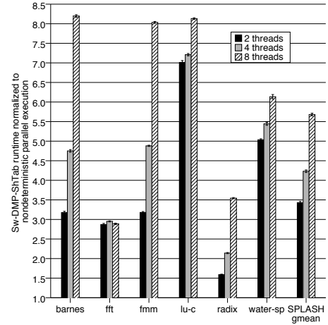
Figure 14. Runtime of Sw-DMP-ShTab relative to nondeterministic execution.
