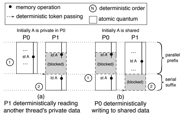
Figure 5. Recovering parallelism by overlapping communication-free execution.
