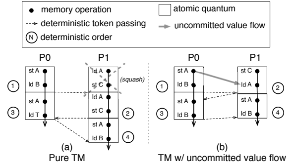
Figure 7. Recovering parallelism by executing quanta as memory transactions (a). Avoiding unnecessary squashes with un-committed data forwarding (b).
