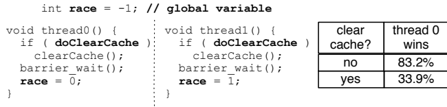
Figure 2. Simple program with a data race between two threads and the outcome of the race with 1000 runs.
