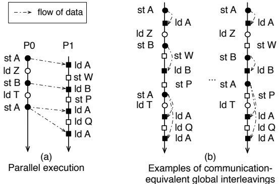
Figure 1. A parallel execution (a) and two of its multiple communication-equivalent interleavings (b). Solid markers represent communicating instructions, hollow markers represent instructions that do not communicate.
