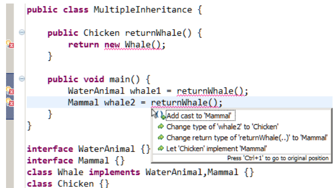
Figure 4. An incompatible return type causes three compilation errors. At the second and third error locations, Quick Fix fails to recommend changing the return type declaration of returnWhale() from Chicken to Whale .
