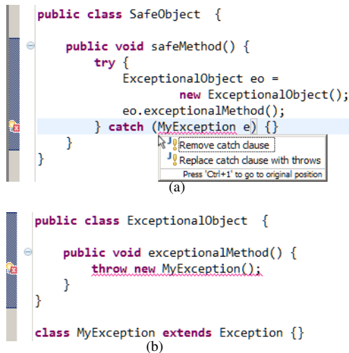
Figure 2. A missing throws declaration causes two compilation errors. At the first error location, Quick Fix fails to recommend declaring exceptionalMethod() to throw MyException .
