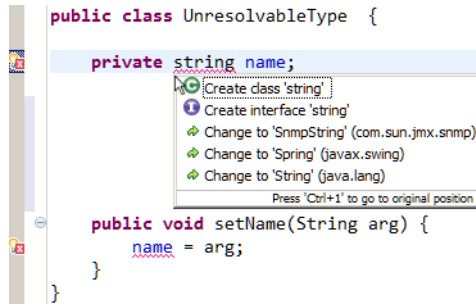
Figure 1. An unresolvable type declaration string causes two compilation errors. At the second error location, Quick Fix fails to recommend changing string to String .
