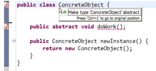
Figure 3. A missing method implementation causes two compilation errors. At the first error location, Quick Fix fails to recommend implementing the body of doWork() .
