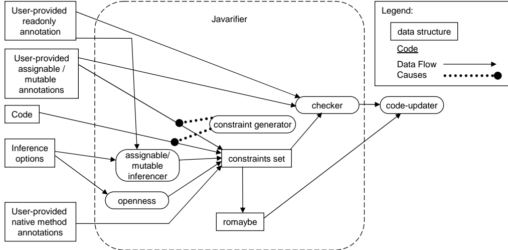
Figure 14: Data flow diagram of Javarifier.
