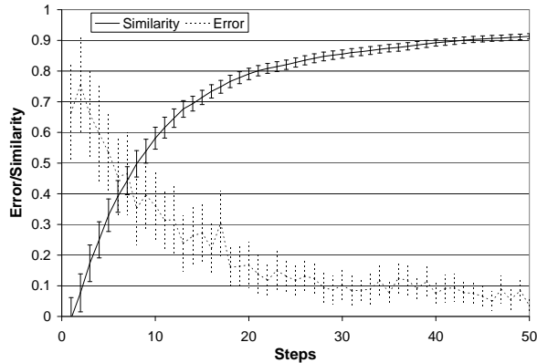
Figure 3: Error and similarity metrics averaged across the first 50 steps of 100 simulated DIAManD runs. There are fifteen attributes and eight choices in the domain. Confidence bars are set to 99% assuming a two-tailed Gaussian distribution of results.
