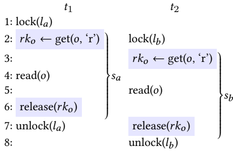
(b) Shared read. t_2 can obtain rk_o to read from o while t_1 is holding rk_o .
