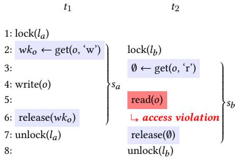
(a) Exclusive write. t_2 cannot obtain a read-only key rk_o to read from o while t_1 is holding a read-write key wk_o .
