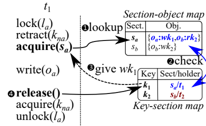
(b) Domain enforcement. Attempt to acquire the keys of objects belonging to s_a when t_1 enters it.
