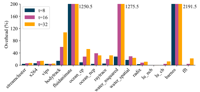
Figure 5: The scalability of KARD while executing PARSEC and SPLASH-2x with 8, 16, and 32 threads.
