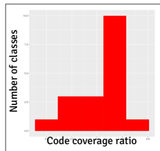
Changed binning
