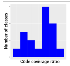
Adequate binning
