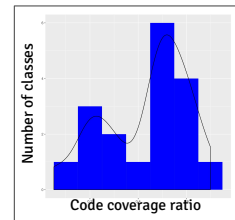
Kernel density overlay
