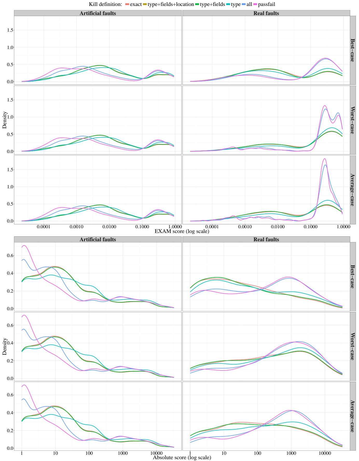
Fig. 4. The effect of the choice of the “Interaction (kill) definition” on MUSE’s EXAM and absolute scores for artificial vs. real faults.
