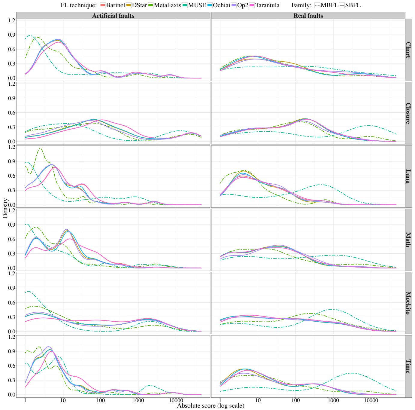
Fig. 6. Distribution of the absolute scores per program for all fault localization techniques and artificial vs. real faults. The absolute score is the location of the defective statement in the suspiciousness ranking of program statements, computed by a fault localization technique.
