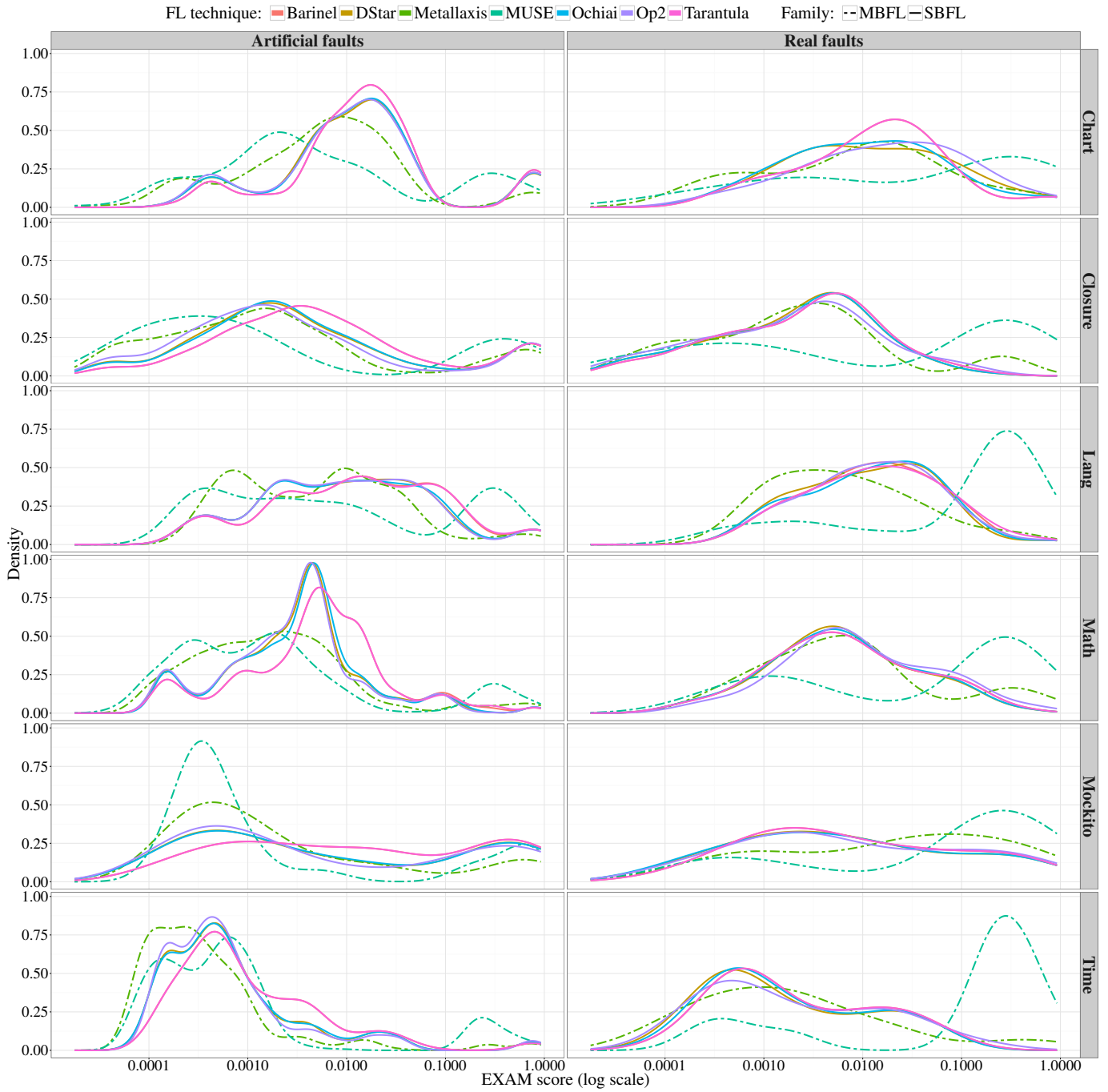
Fig. 5. Distribution of the EXAM scores per program for all fault localization techniques and artificial vs. real faults.
