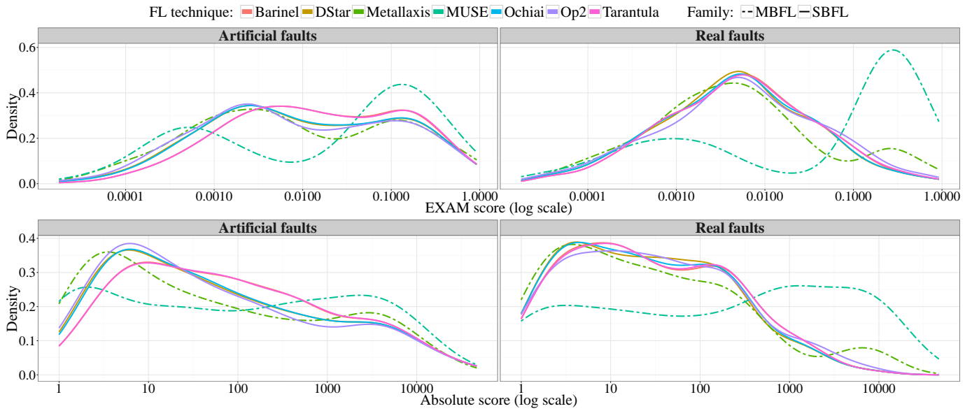
Fig. 7. Distributions of EXAM and absolute scores for all FL techniques, considering the best-case debugging scenario and averaging each FL technique's scores across the artificial faults corresponding to each real fault as described in section V-E. The absolute score is the first location of any defective statement in the suspiciousness ranking of program statements, computed by a fault localization technique.
