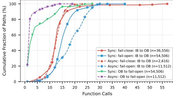
(a) Go call path lengths
