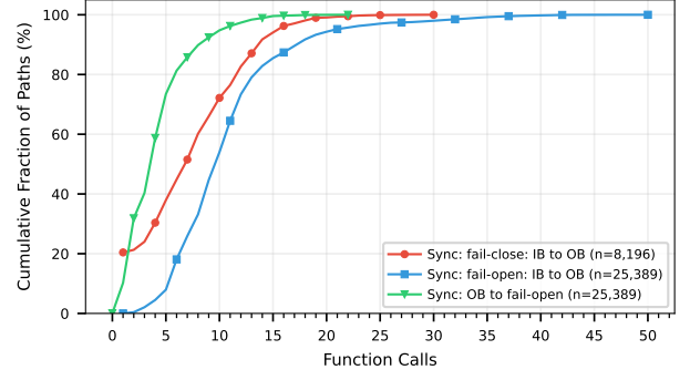
(b) Java call path lengths
