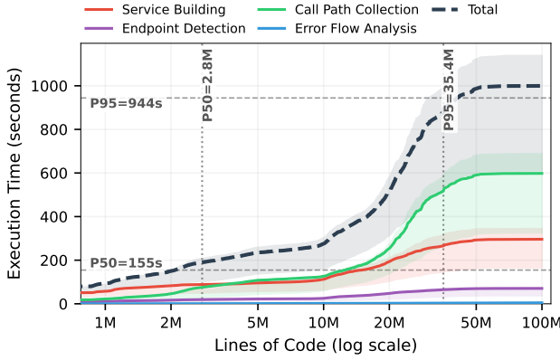
(a) Go analysis execution time.
