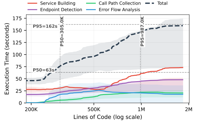
(b) Java analysis execution time.
