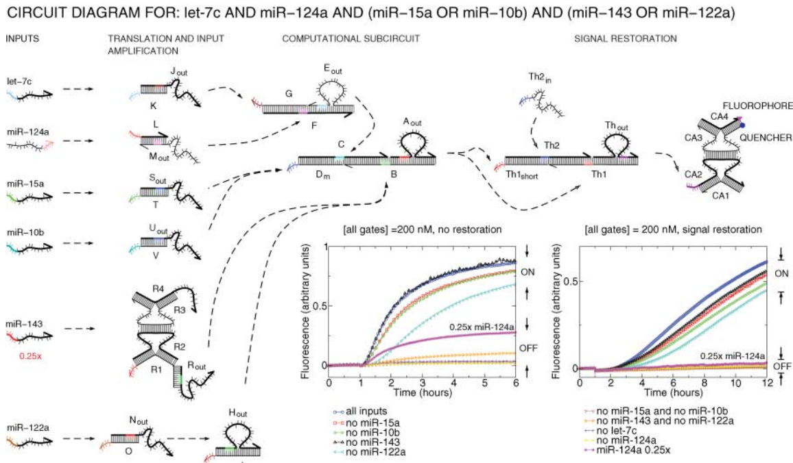
Fig. 3. Signal propagation through a complex chemical circuit combining AND, OR, sequence translation, input amplification, and signal restoration. The five-layer circuit consists of a total of 11 gates and accepts six inputs. With the exception of the threshold gate, which was at 100 nM with its Th 2in strand at 150 nM, all gates were at 200 nM (1×) per gate. Unless otherwise specified, inputs were added at 250 nM (1.25×). miR-143 was added at 50 nM (0.25×) and subsequently amplified by the input amplifier. (Inset) Fluorescence traces of circuit operation without and with the signal restoration module (threshold plus amplifier). The traces for input conditions corresponding to a logical TRUE output (ON) are clearly distinguishable from the logical FALSE output (OFF). Cases tested include when all inputs are present, all cases in which exactly one input is missing, and combinations of inputs that turn off an
