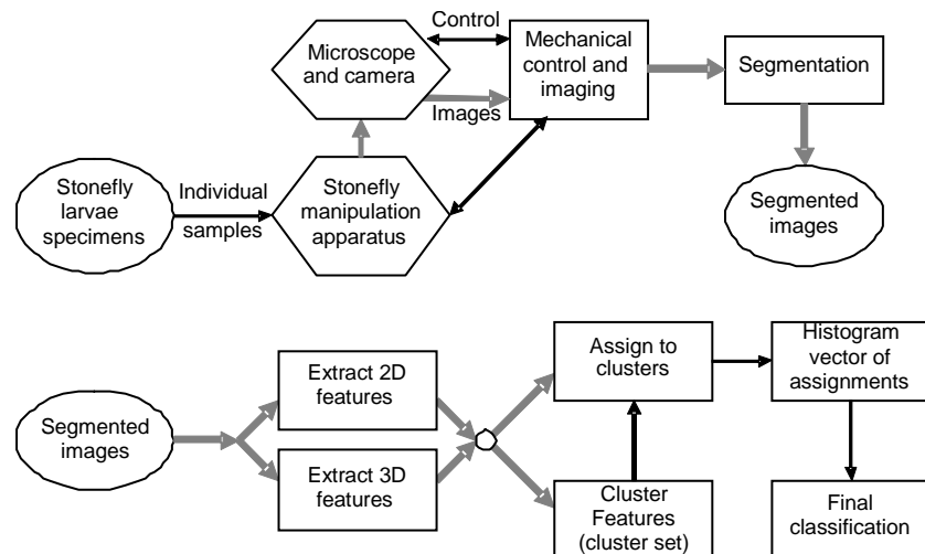
Figure 2. Diagram of stonefly classification system.
