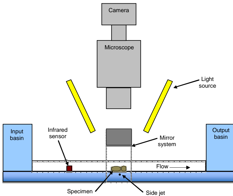
Figure 4. Aquatic insect imaging system.
