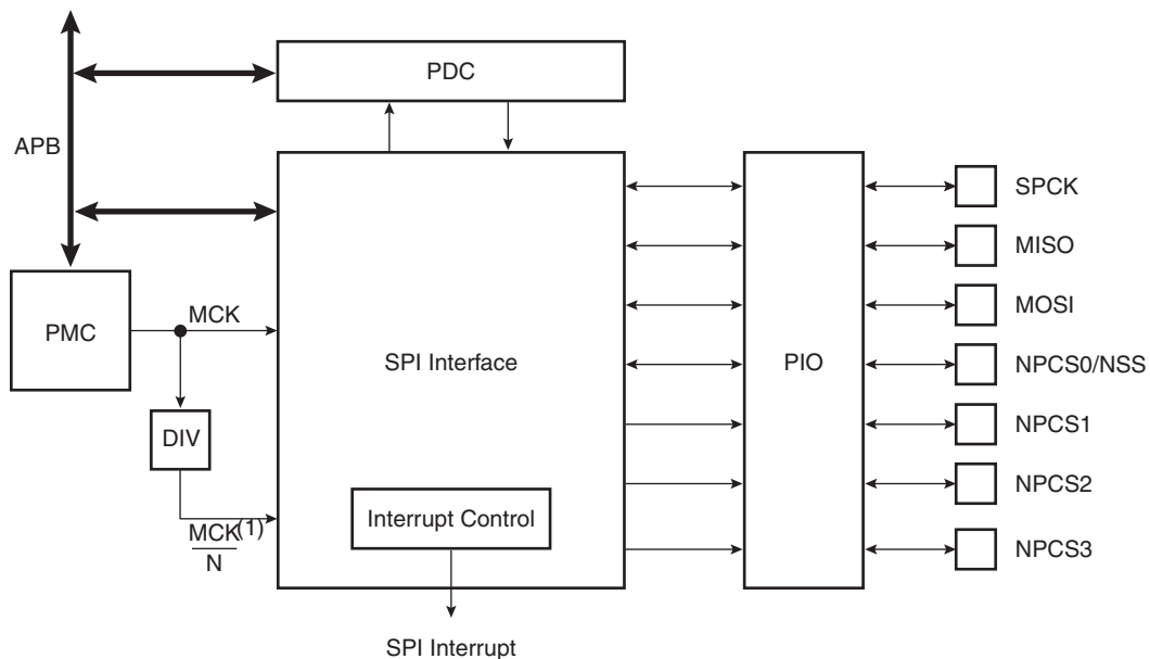
Figure 29-1. Block Diagram
