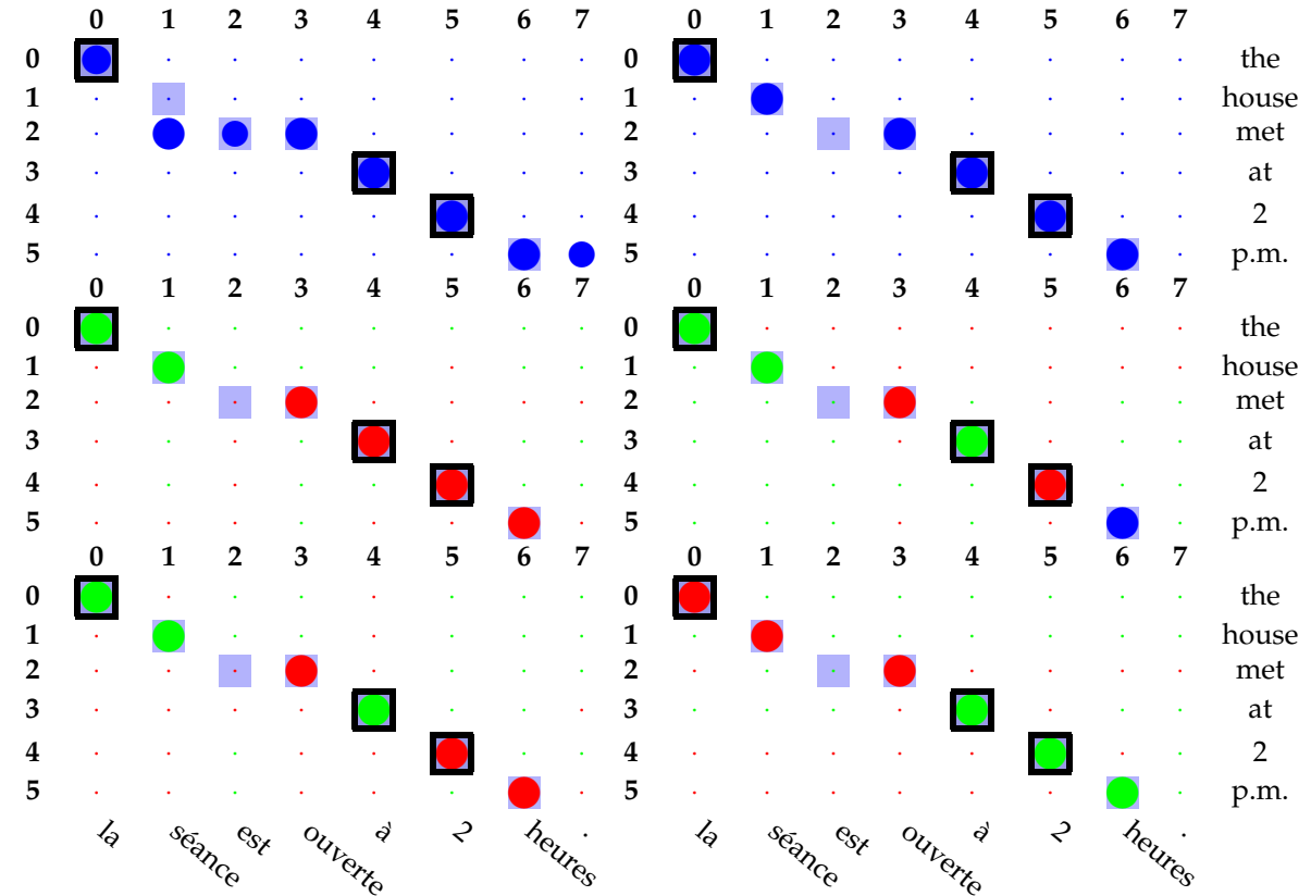
Figure 9 Posterior distributions for different models for English to French sentence. Left: EN→FR model. Right: FR→EN model. Top: Regular HMM posteriors. Middle: After applying the bijective constraint. Bottom: After applying the symmetric constraint. Sure alignments are squares with borders; possible alignments are squares without borders. Circle size indicates probability value. Circle color in the middle and bottom rows indicates differences in posterior from the top row. Green - higher probability, red - lower probability.
