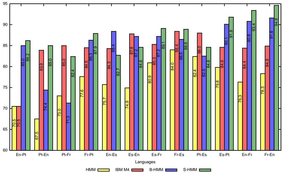
Figure 5 Word alignment precision when the threshold is chosen to achieve IBM M4 recall with a difference of +/- 0.005. The average relative increase in precision (against the HMM model) is 10% for IBM M4, 11% for B-HMM and 14% for S-HMM.
