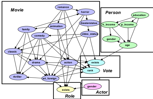
Figure 3. The PRM learned using existence uncertainty.
