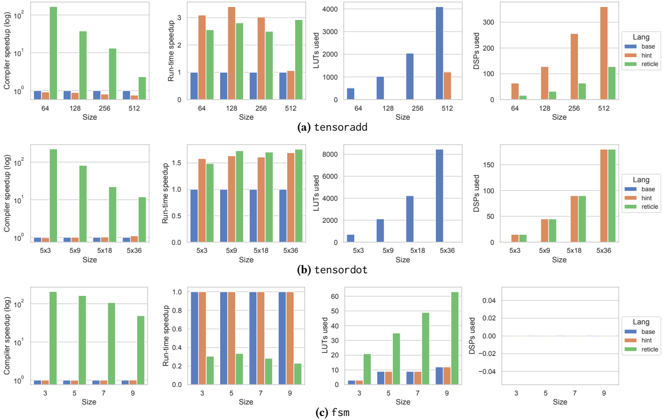
Figure 13. Compiler, run-time, and utilization results of three benchmarks, tensoradd (a), tensordot (b), and fsm (c), when using behavioral Verilog (base), behavioral Verilog with DSP hints (hint), and Reticle (reticle).
